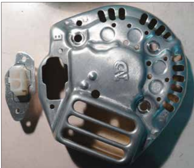
An alternative to having wires coming out of the cover is to mount a Molex-style terminal to the cover and attach it with two pop-rivets.
