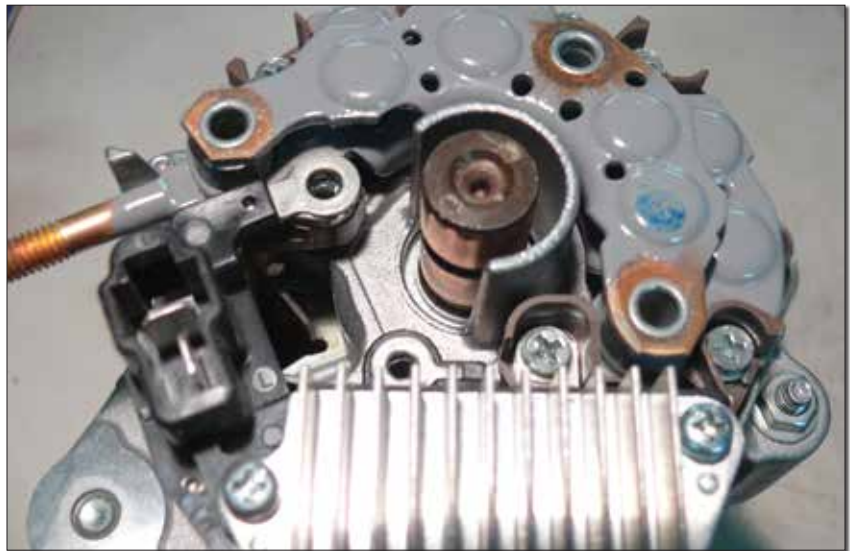
(Left) The brush holder is held in place with two screws. (Right) The alternator after removing the brush holder.
