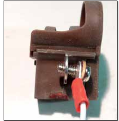
Assemble one fiber washer and the nylon tube on an M4x10-mm screw (left), then add a new wire terminal with a 5-mm hole, and fit the screw into the now 5-mm hole in the brush holder.
