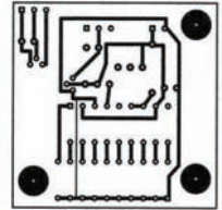
(right) Top, bottom and overlay PC board layout.
